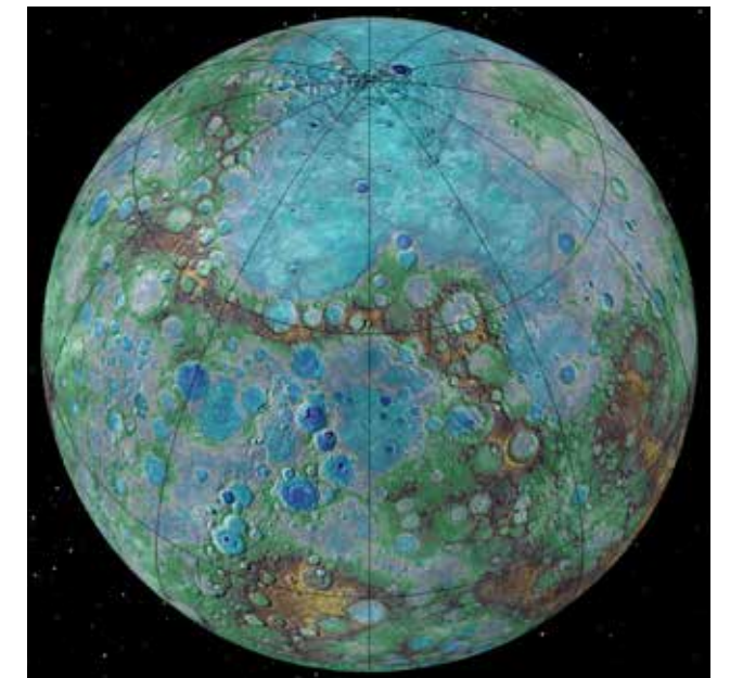
National Air and Space Museum Senior Scientist Thomas R. Watters determined that Mercury is tectonically active, joining Earth as the only two such planets in our solar system. Watters' finding comes through his participation in NASA's MESSENGER Mercury spacecraft team.
